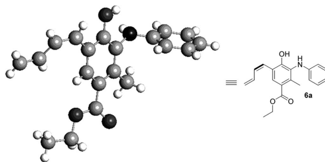
Figure 1. Crystal structure of ethyl ( Z )-5-(buta-1,3-dienyl)-4-hydroxy-2-methyl-3-(phenylamino)benzoate ( 6a ).
