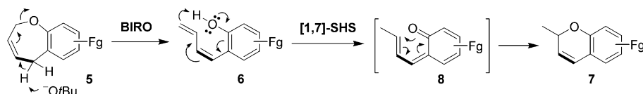
Scheme 1. Proposed reaction mechanism.
